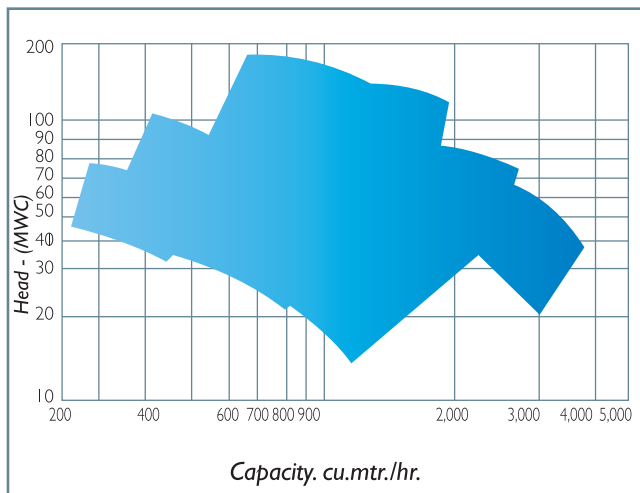
Horizontal Split Case Pump "WLN" - Heavy Duty Series Coverage Chart 4 Pole 50Hz
