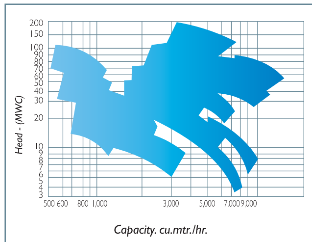
Horizontal Split Case Pump "WLN" - Heavy Duty Series Coverage Chart 6, 8 & 10 Pole 50Hz
