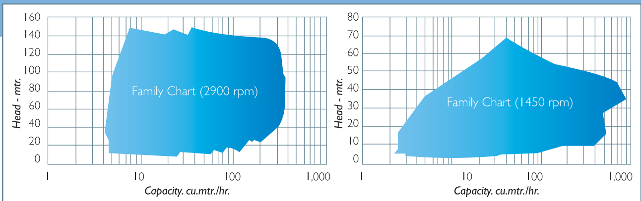
Chart of WPE - End Suction Pump - ISO 2858
